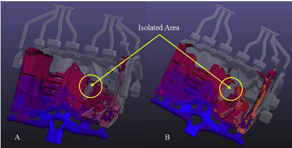
Fig. 5. Simulation results after 40% filling. (A) Case 1, (B) Case 2.
