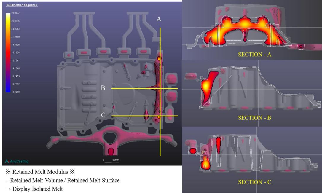
Fig. 9. Expected shrinkage defect areas of Case 3.
